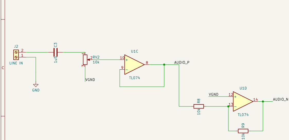
C Input stage (level -> buffer -> inverter)
