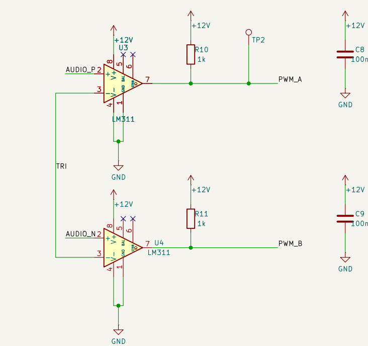
D PWM comparators (audio vs triangle)
